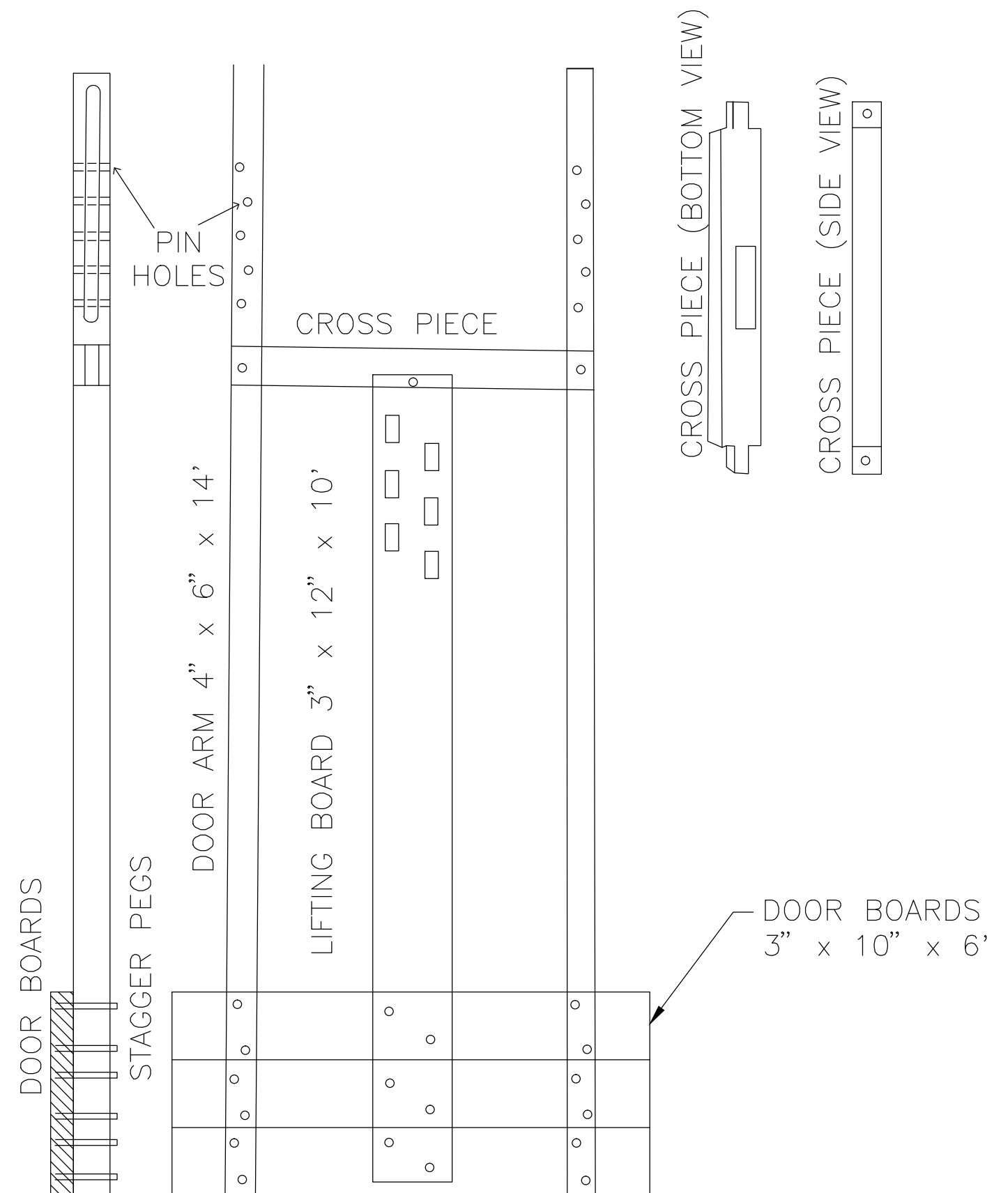
3 FLAPGATE (FRONT VIEW) (NOT TO SCALE)
